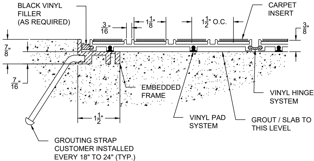
SECTION A
