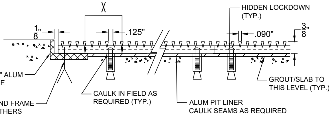
SECTION A
