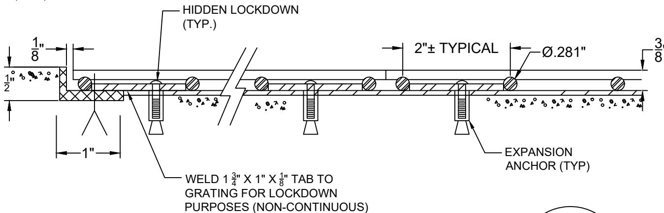
SECTION B
