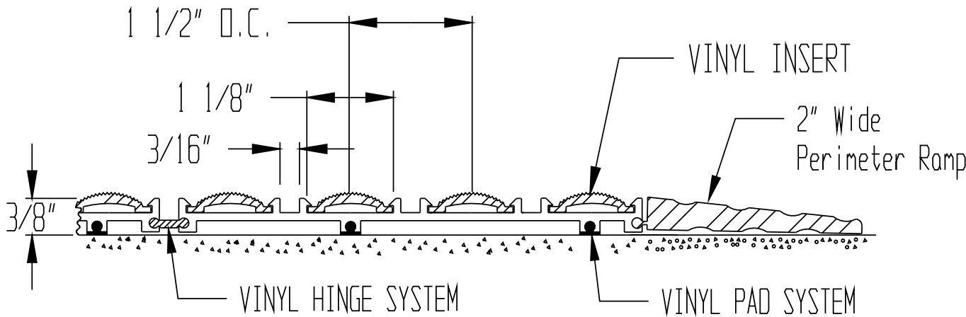
SECTION A
