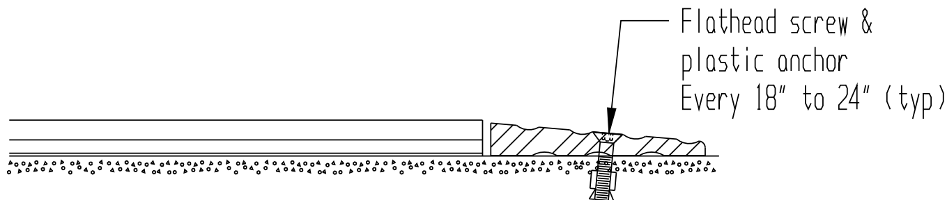
SECTION B
