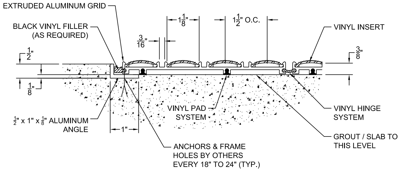
SECTION A
